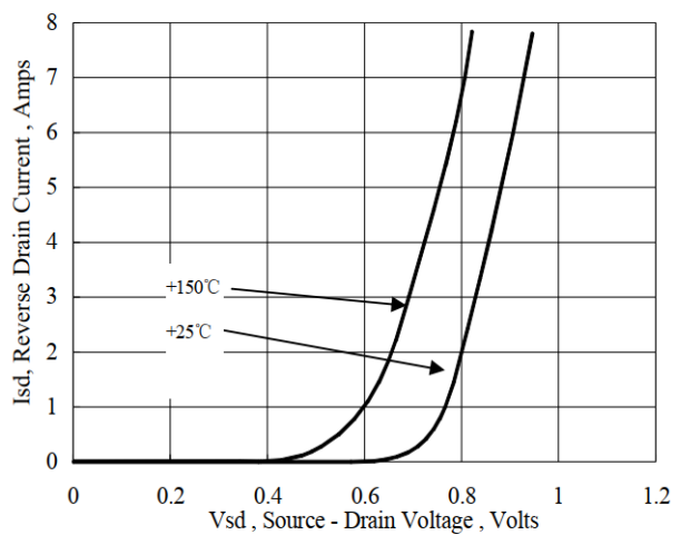
Fig 6 Body-Diode Characteristics
